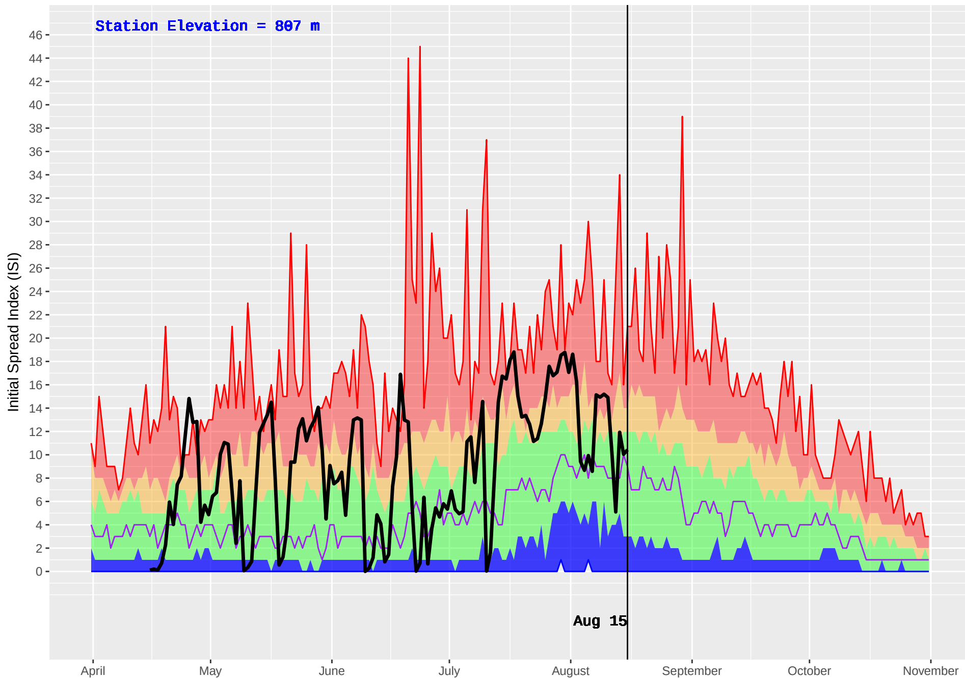
BEAVERDELL (390) : Historical (1970–2016) and Current (2018) Daily Initial Spread Index (ISI)
